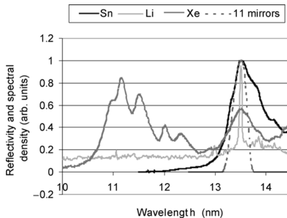
Figure 2.2 Calculated near-normal-incidence reflectivity of an 11-mirror system, based on the model of CXRO, 11 vs. spectra of Sn, Li, and Xe, as acquired in a joint investigation by ASML-ISAN. 8
