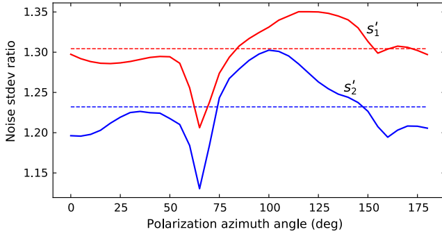
Fig. 3 The increase (multiplying factor) in the normalized Stokes parameter standard deviations \text{std}(\hat{s}'_1) and \text{std}(\hat{s}'_2) with respect to the input polarization angle, where the increased noise is caused by applying the correction of Eq. (9). The dashed lines indicate the average standard deviation ratio taken across all angles.
