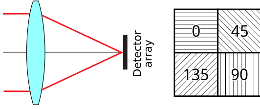
Fig. 1 A polarization camera showing a 2 \times 2 pixels group from the detector array and their polarization filter orientations.
