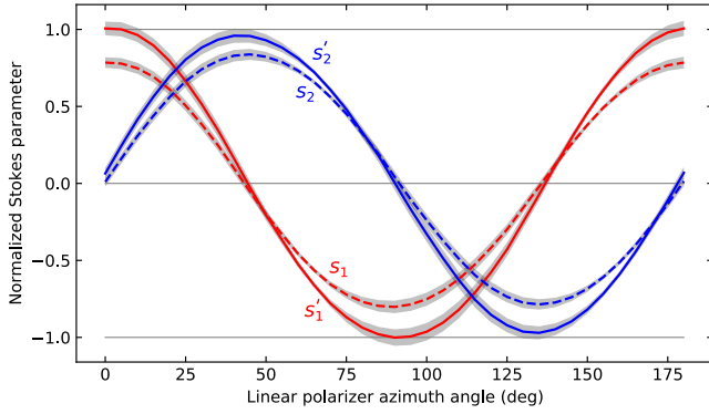
Fig. 2 The measured uncorrected linear Stokes parameters \hat{s}_1 and \hat{s}_2 and corrected parameters \hat{s}'_1 and \hat{s}'_2 obtained while rotating the input angle of polarization from 0 deg to 180 deg. Note that the Stokes parameters, here, are shown in their normalized form: s_1 = s_1/s_0 and s_2 = s_2/s_0 . Each curve is obtained as an average of the results from all pixels of the camera, while the grayed regions astride each curve give the standard deviation of the result, also calculated using all pixels on the camera. The dashed curves indicate the measurement result using the ideal polarization analysis matrix [Eq. (4)] and the solid curves give the measurement with the corrected analysis matrix [Eq. (10)].
