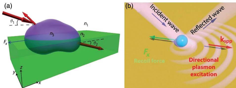
Fig. 6 OPF realized on an interface. (a) Optical pulling on an air–water interface, which is realized by the linear momentum increase when the incident light is scattered from air to water through the object. 38 (b) Optical pulling on a plasmonic surface, which is realized by the directional excitation of the SPP on the air–silver interface. 75
