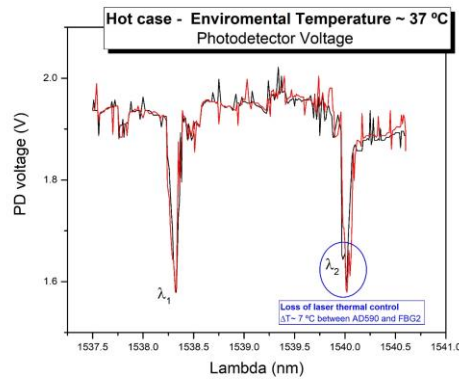
Figure 7: Raw telemetry data in hot case where T= 37 \text{ }^\circ\text{C} : AD590 temperature during CM upload (up left), laser thermistor temperature (up right) during CM upload and PD voltage with respect to \lambda_{\text{las}} (down). Note the loss of thermal control of the laser.
