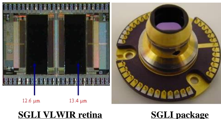
Figure 2-8 : SGLI detector
