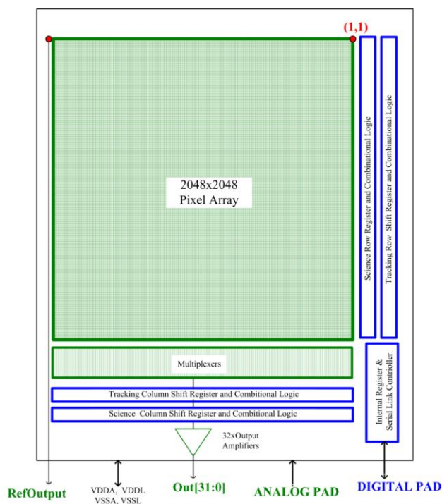
Figure 3-1 : ALFA ROIC architecture
