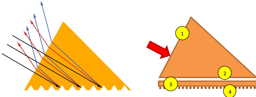
Figure 1 On the left the immersed grating principle is shown: light enters the prism through a polished entrance facet; after diffraction at the grating facet the dispersed light leaves the prism through the same facet. On the right the WFE contributors of the immersed grating are listed. The entrance surface is indicated with the arrow. #1 is the WFE of the front surface of the prism. #2 is the WFE of the back surface of the prism (before fusion of the prism with the wafer containing the grating). #3 is the WFE that results from the wafer total thickness variation (TTV, before fusion with the prism) and #4 is the WFE of the grating in reflection as measured from the air side of the grating. Material inhomogeneity is considered negligible.
