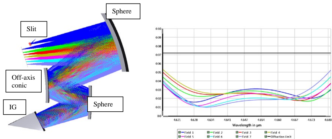
Figure 6 Layout (left) and RMS WFE in waves (right) of the proposed IG based spectrometer after the last optimization step. Diffraction limit is indicated by a horizontal line.
