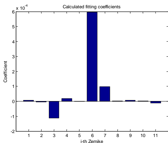
Figure 8 The Zernike decomposition of the surface deformation (Figure 7) is shown. The coefficients show the RMS surface deformation of each Zernike term in mm. The most dominant aberration is astigmatism (RMS 0.6 \mu\text{m} surface deformation).
