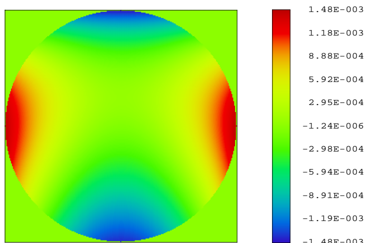
Figure 7 The surface deformation of the grating looking from Littrow direction is shown. It is the result of a variable (x,y) grating pattern that creates these low order aberrations. The units are in mm. The PV surface deformation is less than 3 \mu\text{m} .
