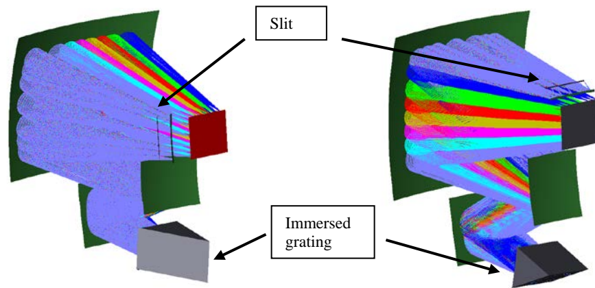
Figure 2 Layout of two IG based designs. On the left the slit and the detector are next to each other on the right they are in the plane of the TMA mirrors.
