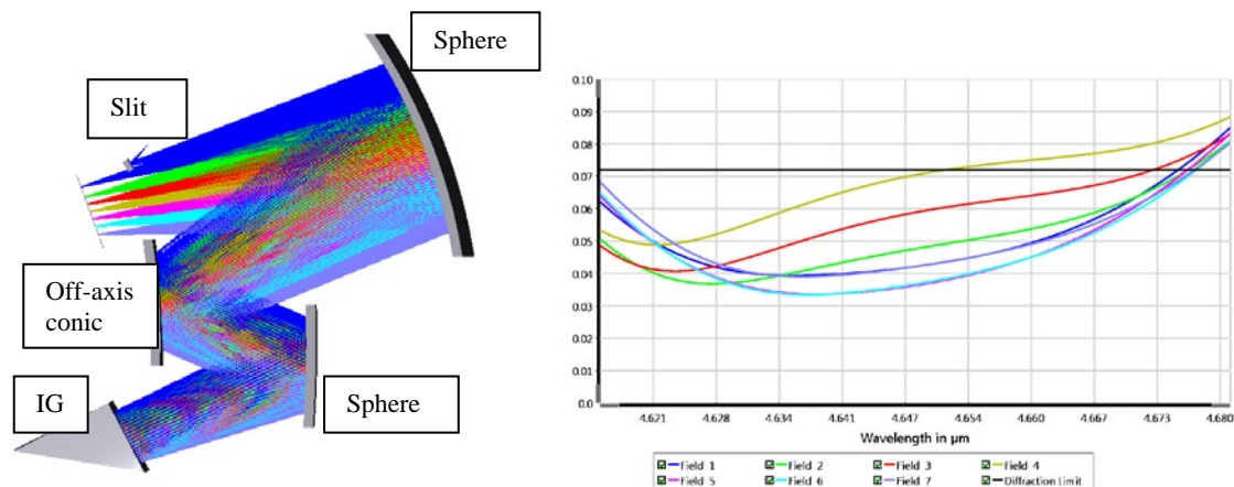
Figure 5 Layout (left) and RMS WFE in waves (right) of the proposed IG based spectrometer after the second optimization step. Diffraction limit is indicated by a horizontal line.
