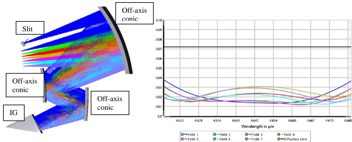
Figure 4 Layout (left) and RMS WFE in waves (right) of the proposed IG based spectrometer after the first optimization step. Diffraction limit is indicated by a horizontal line.
