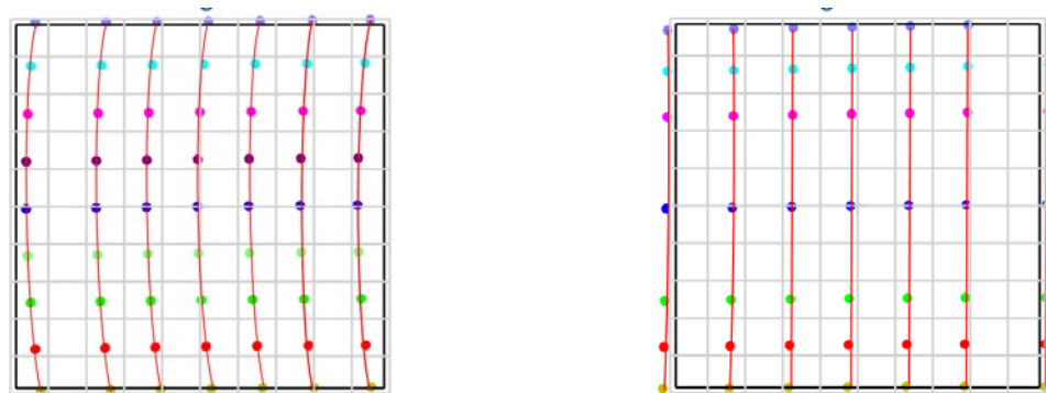
Figure 3 The slit geometry is shown for the two designs presented in Figure 2. By arranging the detector and the slit in the plane of the three mirrors of the TMA, straight slit geometry can be achieved.
