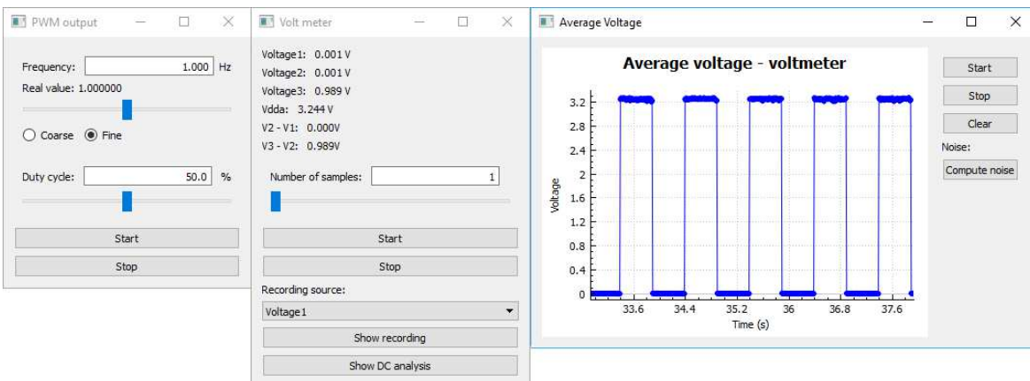
Figure 2. F0 – LAB user interface (PWM output and Voltmeter shown)
