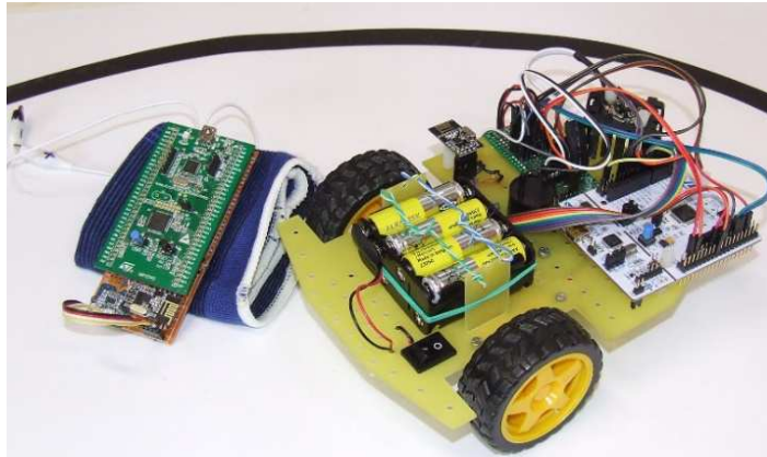
Figure 4. Remotely controlled MiniRover
