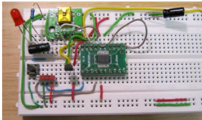
Figure 1. F0 - LAB platform connection in the solderless contact field (breadboard).
