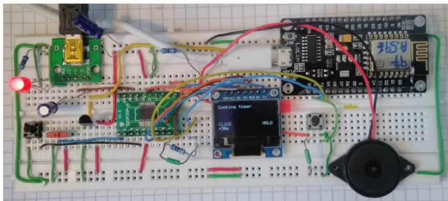
Figure 3. Kitchen timer based on STM32F042 microcontroller
