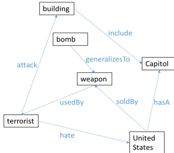
Fig. 8. Reasoning systems need to be able to give approximate answers when exact answers are impossible. Through sparse matrix techniques the intelligent agent is able to approximate reasoning with partial information and expand the knowledge base by exploiting distributional semantics at query time. In this simple example, terrorist is linked to Capitol [41].
