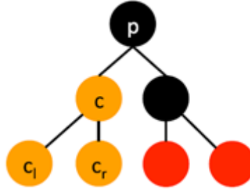
Figure 3. Illustration that depicts the relationships for group c in a local neighborhood of H, including its parent p and left and right children, c l and c r . [30]
