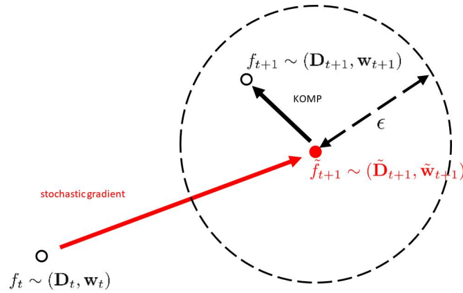
Figure 2. Visual depiction of POLK where epsilon is the size of the error neighborhood and f_t is the current data point, \tilde{f}_t is the estimate of the next SGD step and f_{t+1} is the POLK estimate. D_t is the kernel dictionary. The function f_t is parameterized by dictionary D_t and weight vector w_t . f_{t+1} is determined from output of DKOMP on \tilde{f}_{t+1} which is parameterized by (\tilde{D}_{t+1}, \tilde{w}_{t+1}) [18].
