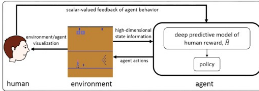
Figure 6. The Deep TAMER framework. A human observes an autonomous agent trying to perform a task in a high-dimensional environment and provides scalar-valued feedback as a means by which to shape agent behavior. Through the interaction with the human, the agent learns the parameters of a deep neural network, \hat{H} , that is used to predict the human's feedback. This prediction then drives the agent's behavior policy. [36]
