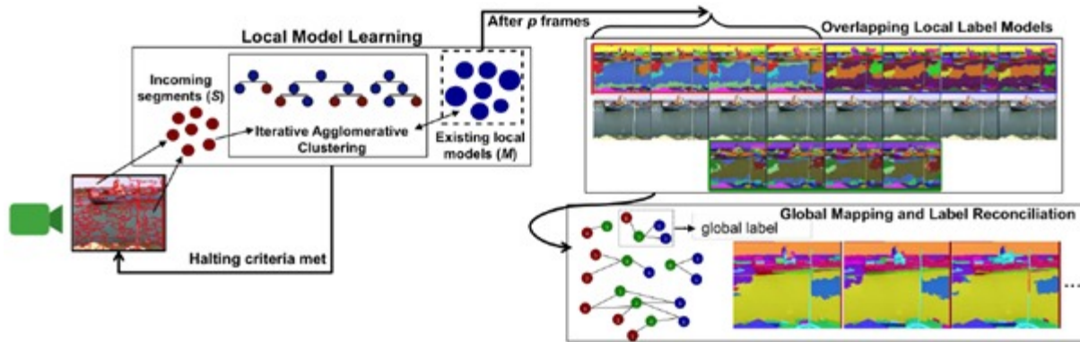
Figure 5. Overview of the USSL algorithm. The next image from the data stream is over-segmented, and segments are agglomeratively merged with existing models from previous frames in the stream. Overlapping local models are created for a window in the stream and these local label sets are mapped and reconciled using a graph encoding to generate a global label set. [32]
