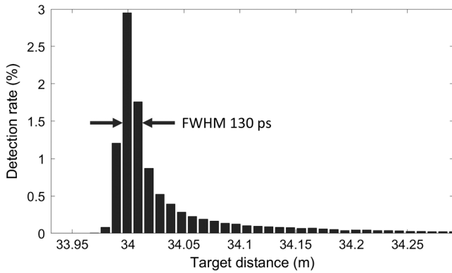
Fig. 11 Detection rate with the target at 34 m.
