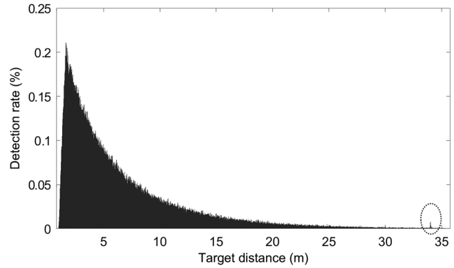
Fig. 13 Detection rate with the target at 34 m and a wide time gate.
