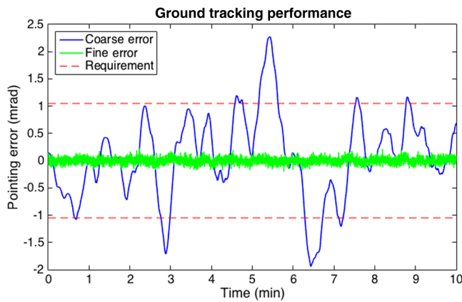
Fig. 5 Coarse and fine stage pointing error with beacon feedback and compensation for environmental disturbances, from Ref. 28.
