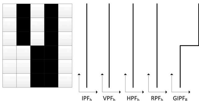
Fig. 3 Scenario in which GIPF_R is better than IPF_h , VPF_h , and HPF_h in capturing horizontal variation. Each grid represents a pixel or several pixels.
