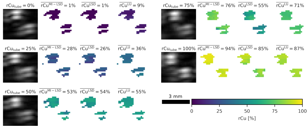
Fig. 10 Example ROI in the phantom test set B with the estimation results for MI-LSD, LSD, and LU. Shown are the lower two tubes of a four tube phantom with SVF = 0.5\% and rCu_{bg} = 25\% . To indicate the content of the ROI, the mean OA signal in the ROI is shown left, with the ground truth rCu_{tube} annotated. The brightness of the OA signal is independently and linearly autoleveled for each ROI. The mean rCu estimate \overline{rCu} over the ROI is noted for the three estimators.
