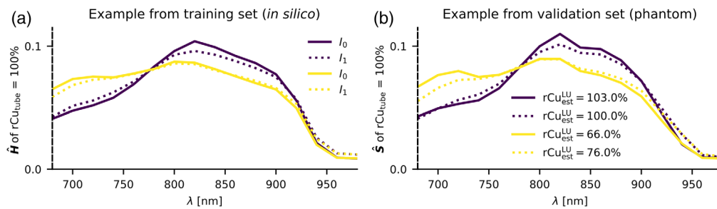
Fig. 6 Examples for spectral coloring in L1 normalized spectra of an absorber with r\text{Cu}_{\text{tube}} = 100\% . Comparison between (a) in silico absorbed energy spectra \hat{\mathbf{H}} and (b) phantom OA signal spectra \hat{\mathbf{S}} . Spectra for two background media are shown: r\text{Cu}_{\text{bg}} = 100\% (yellow), r\text{Cu}_{\text{bg}} = 0\% (dark); with \text{SVF} = 1\% . The spectra for two illumination positions I_0 (line) and I_1 (dotted) are shown as an example for two of the four illuminations. Systematic changes in the spectral coloring can be seen for different background media and illumination positions. These changes are qualitatively similar for \hat{\mathbf{H}} and \hat{\mathbf{S}} . On the validation phantom examples LU estimations for single spectra r\text{Cu}_{\text{est}}^{\text{LU}} are listed—spectral coloring can cause large estimation errors relative to the r\text{Cu}_{\text{tube}} = 100\% ground truth.
