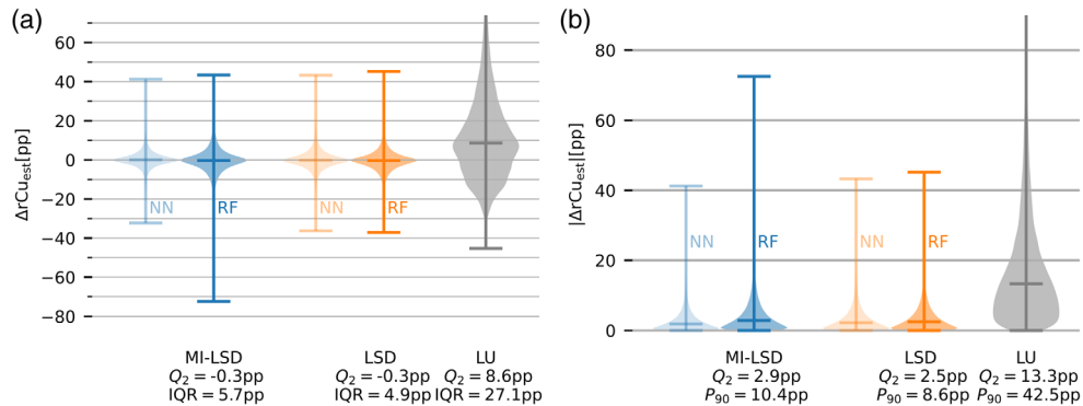
Fig. 8 Error distributions of the in silico rCu test set cf. Fig. 5. (a) rCu estimation errors \Delta rCu_{est} and (b) their absolutes. Blue shows the rCu estimators using MI-LSD, orange the estimators using LSD, and gray is the LU reference. Medians Q_2 of the error distributions are shown, together with interquartile ranges (IQR) and 90th percentiles P_{90} . The two feedforward NN models and the two RF models all have median absolute errors below 3 pp.
