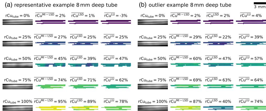
Fig. 11 Example ROI 8 mm deep in the phantom test set C with estimation results for MI-LSD, LSD, and LU. Shown are two ranges of five imaged tubes with their rCu_{\text{tube}} annotated above their mean OA signal. The brightness of the OA signal is independently and linearly autoleveled for each ROI. The mean rCu estimate \overline{rCu} over the ROI is noted for the three estimators. The ROIs for two sets of phantoms are shown. (a) A representative result ( rCu_{\text{bg}} = 100\% , 1% SVF background), (b) a result with outlier estimation errors (0% SVF background). LSD has highest estimation errors in deep vessels and in phantoms with no added sulfates in the background medium, i.e., in (b) for rCu_{\text{tube}} = 100\% .
