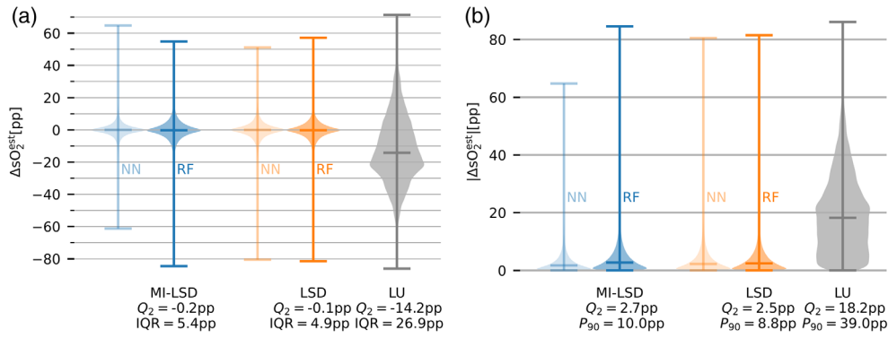
Fig. 9 Error distributions of the in silico sO_2 test set cf. Fig. 5. (a) sO_2 estimation errors \Delta sO_2^{est} and (b) their absolutes. Blue shows the sO_2 estimators using MI-LSD, orange the estimators using LSD and gray is the LU reference. Medians Q_2 of the error distributions are shown, together with IQR and 90th percentiles P_{90} . The two feedforward NN models and the two RF models all have median absolute errors below 3 pp.
