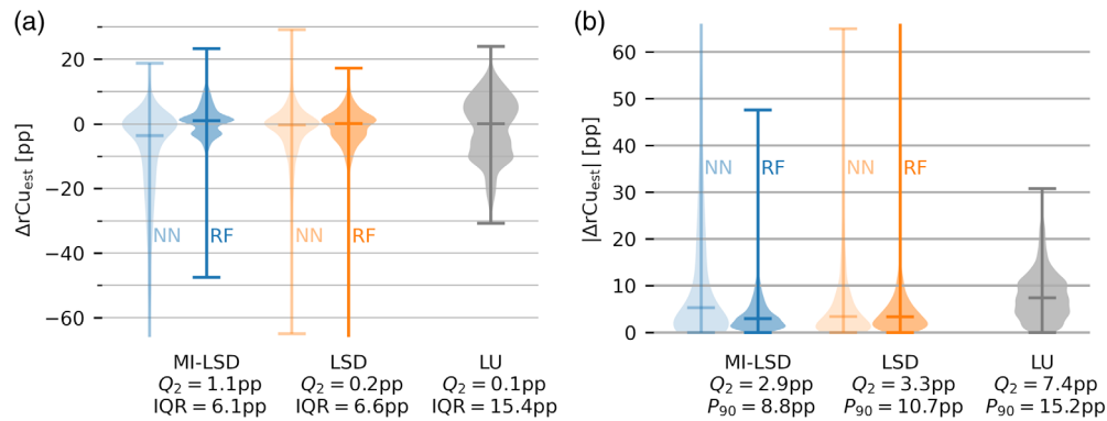
Fig. 12 Error distributions of the phantom test set B [cf. Fig. 4(b)]. (a) rCu estimation errors \Delta rCu_{\text{est}} and (b) their absolutes. Blue shows the rCu estimators using MI-LSD, orange the estimators using LSD, and gray is the LU reference. Medians Q_2 of the error distributions are shown, together with IQR and 90th percentiles P_{90} . The feedforward NN models performed similar to the RF models for the LSD method but underperformed for MI-LSD.
